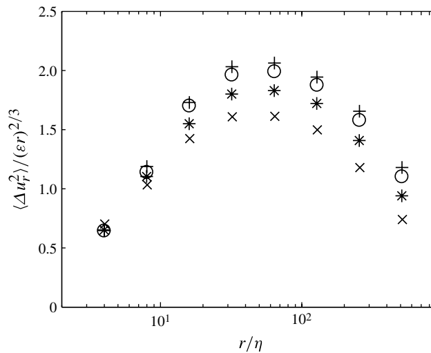
FIGURE 11. Second-order compensated structure functions for the experiments with varying duty cycle: 100% (+), 75% (○), 50% (*), 25% (×). The driving frequency modulations are (f_{high} - f_{low}) = (3-0) Hz and the period T is 30 s.
