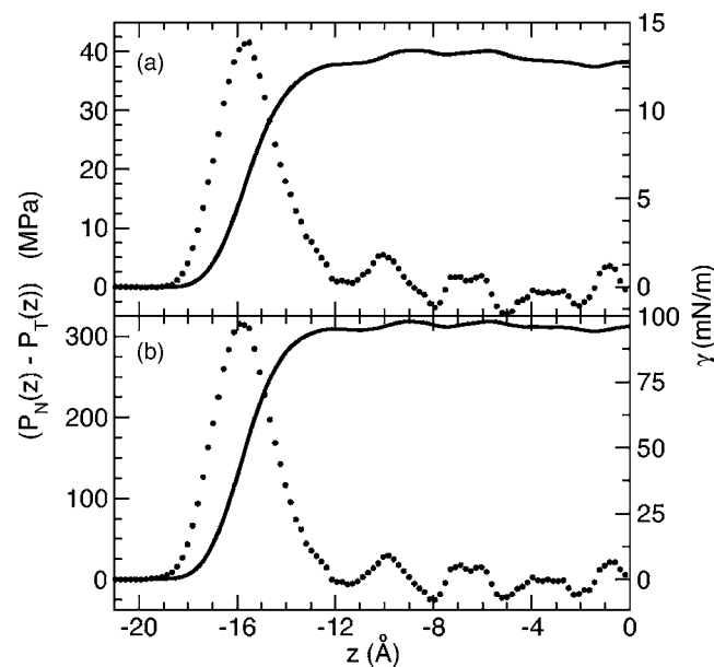
FIG. 7. (a) P_N(z) - P_T(z) is shown in the left axis. Circles represent the profile of the differences between the normal and tangential pressures due to induced-induced dipole interactions. \gamma is shown in the right axis. Continuous lines represent the profiles of \gamma . (b) Axes are the same as (a). Circles represent the profile of the differences between the normal and tangential pressures due to permanent-induced dipole interactions. Continuous line represents the profile of \gamma .
