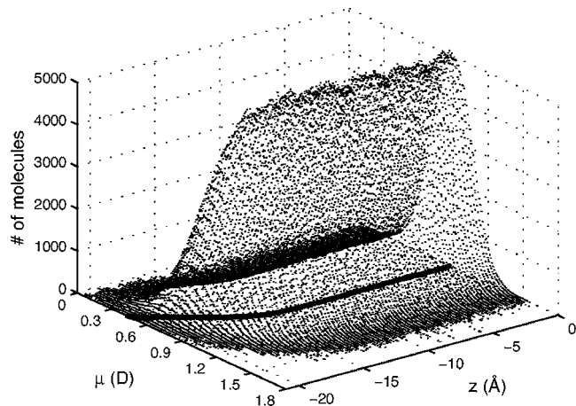
FIG. 5. Histograms of the magnitude of the induced dipole, \mu , of water as a function of the distance from the center of the slab. The figure shows the left interface up to the center of the bulklike region. The heavy line shows the mean induced dipole as a function of z .
