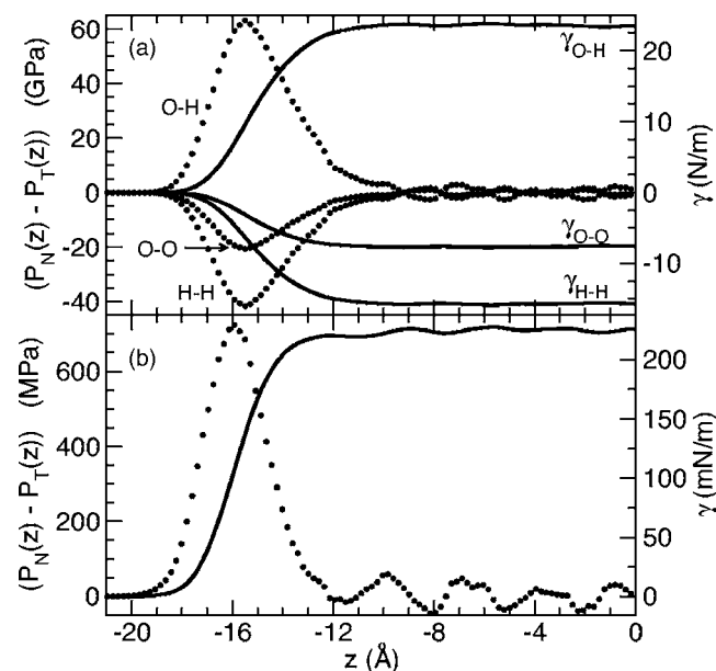
FIG. 6. (a) P_N(z) - P_T(z) is shown in the left axis. Circles represent the profile of the differences between the normal and tangential pressures due to Gaussian distributed charge interactions. \gamma is shown in the right axis. Continuous lines represent the profiles of \gamma . (b) Axes are the same as (a). Circles represent the profile of the differences between the normal and tangential pressures due to the net contribution of Gaussian distributed charges interactions. Continuous line represents the profile of \gamma .
