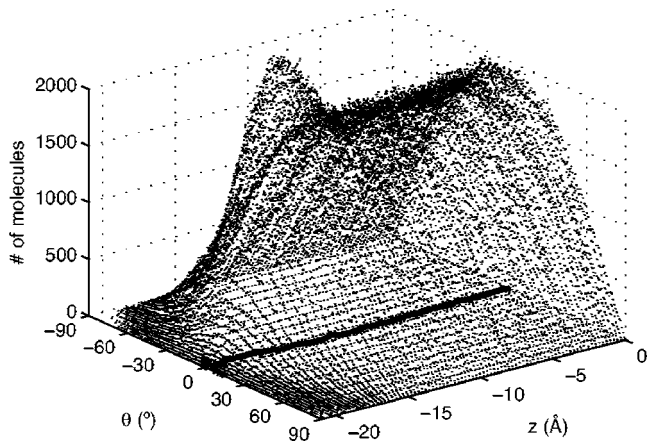
FIG. 4. Histograms of the orientation of the induced dipole of water as a function of the distance from the center of the slab. The figure shows the left interface up to the center of the bulklike region. The heavy line shows the mean angle as a function of z .
