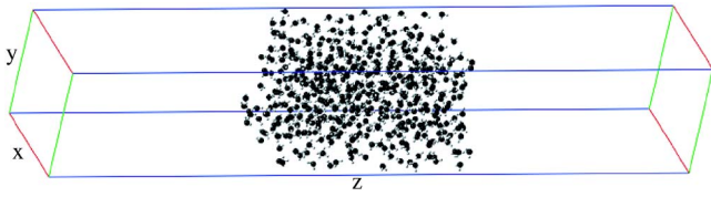
FIG. 1. Snapshot of the simulated system: A slab of liquid water formed by 500 molecules is surrounded by vacuum at 298.15 K. The parallelepiped represents the actual size of the simulation cell.
